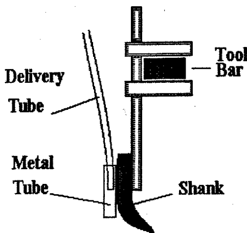
Figure 1 - Shank Setup
